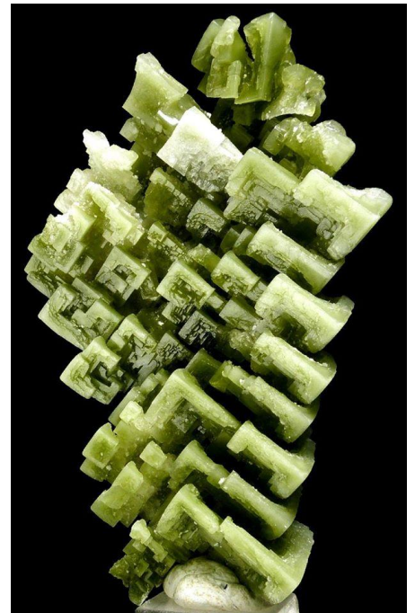
Halite hopper crystals - POLAND.
