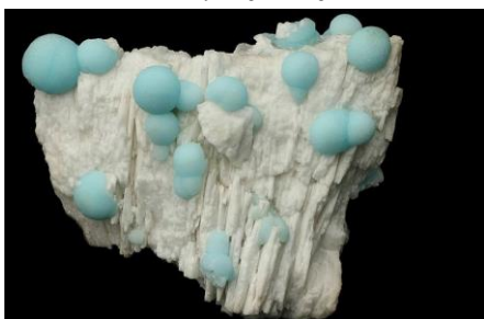
Aragonite on Baryte - Brixlegg, Tyrol, AUSTRIA.
